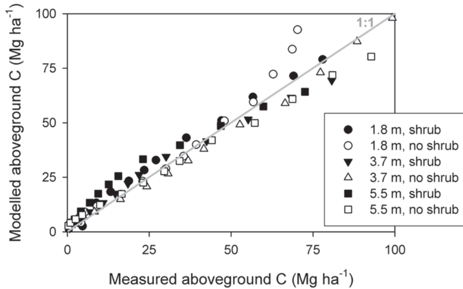
Figure 5 —The relationship in aboveground tree carbon between modeled with 3-PG and calculated from measured DBH on three spacings split with either shrub present or shrub absent plots at the Challenge Initial Spacing study, Challenge Experiment Forest, California.
